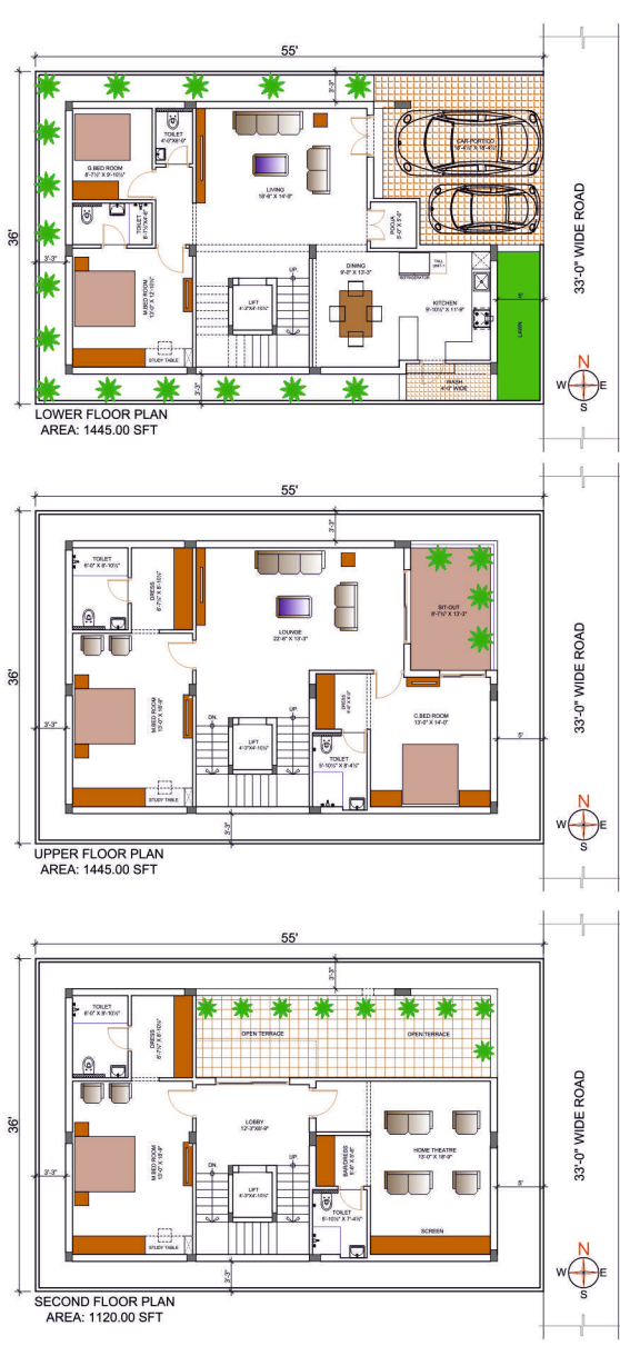
WEST FACING PLAN
