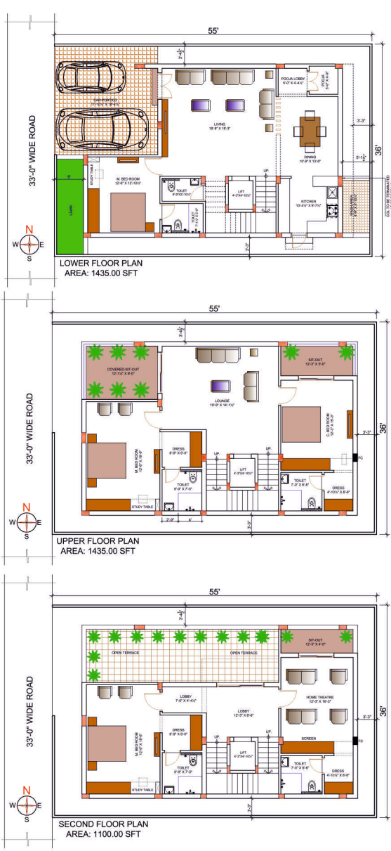
EAST FACING PLAN
